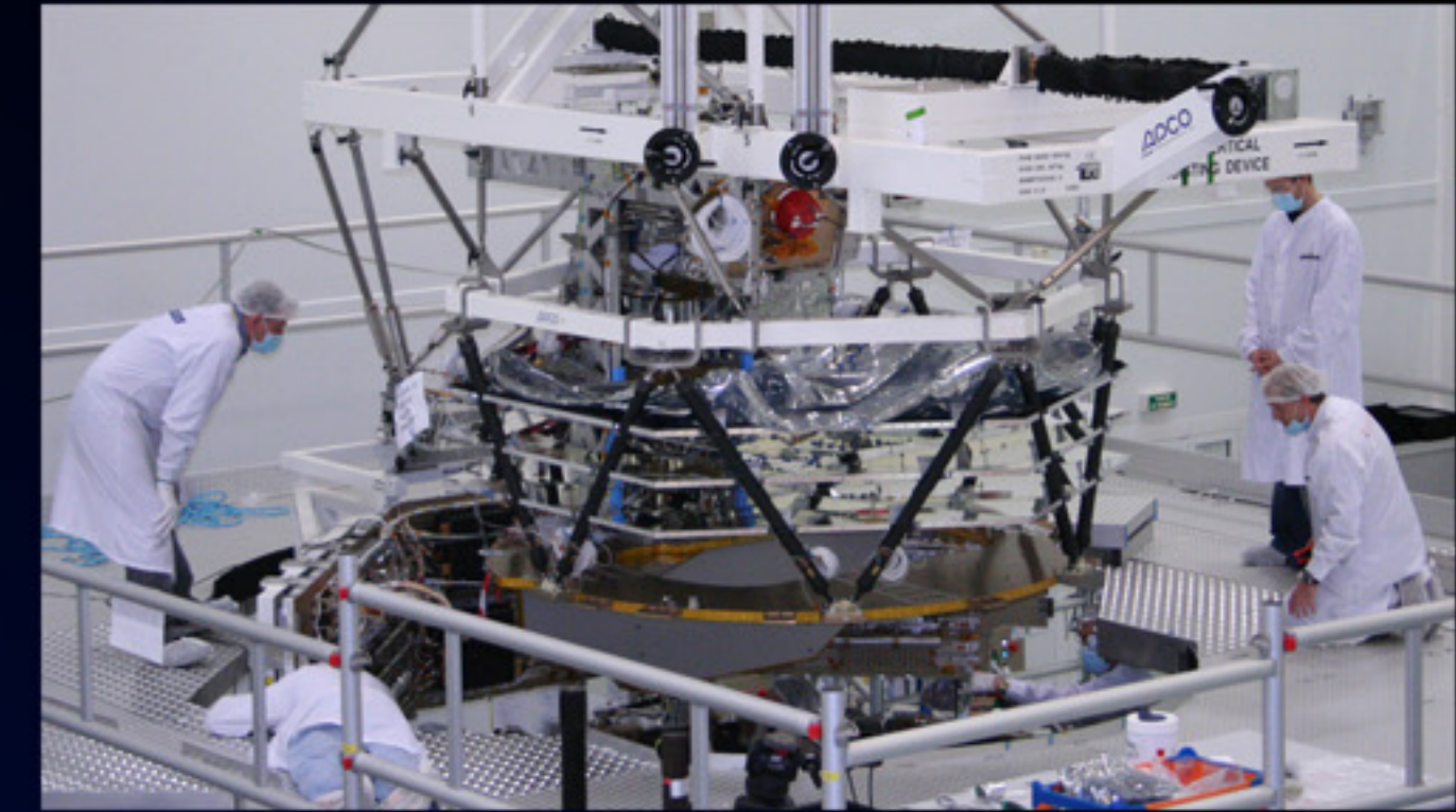
Planck spacecraft in clean assembly at Alcatel Alenia Space in January 2007
